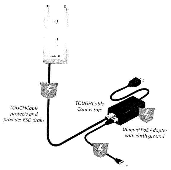
Ubiquiti PoE Adapters and TOUGH Cable protect against ESD events in a network.
