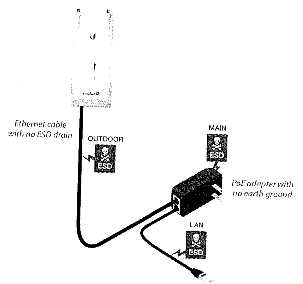
Areas vulnerable to ESD events in a network without a Ubiquiti PoE Adapter.
